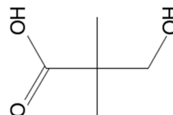
HYDROXYPIVALIC ACID
