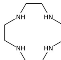
CYCLEN
