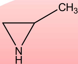
PROPYLENE IMINE
