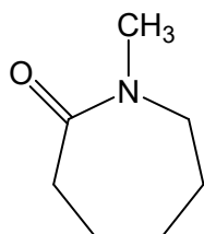
N-METHYL CAPROLACTAM
