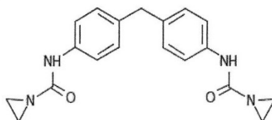
POLYUREA
